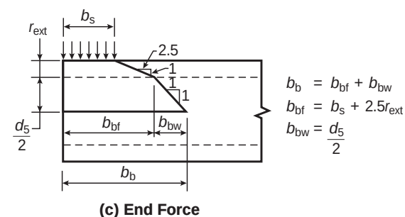
Figure 5.2: Dispersion of force through flange, radius and web of RHS/SHS
